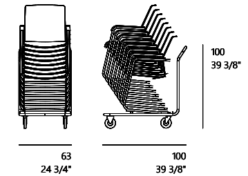
175/71 with headrest
