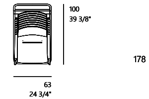
178 Four-wheeled trolley
